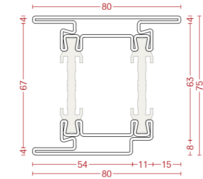
FT 7550H-02 FT 7550H-05 FT 7550H-07 FT 7550H-12
