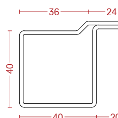
MF 4040LR D
