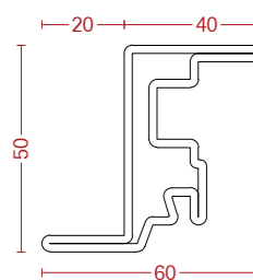
MF 5020ZG A/R Z PROFILE FOR TILT AND TURN
