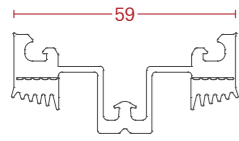
CW GD6074 MULLION (FACADE) OUTSIDE CORNER 3°-15°
